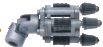
TYPE-5 Wing Arm Head with Universal Joint Range: 1-3/4 in. (44.4 mm) - 13-1/4 in. (336.5 mm) Self feeding Deposit: 1/2 in. (12.7 mm) - thick-hard to medium
